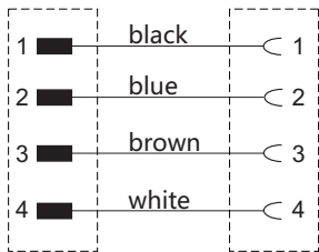
Circuit diagram/电路图
