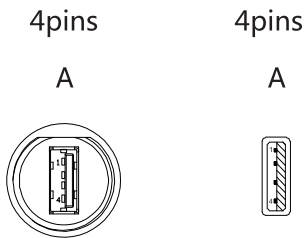
Contact layout/针孔排布 (Front view/前视图)
