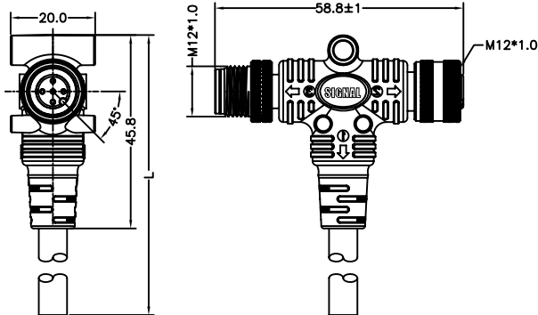
Scale diagram
