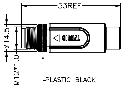
Scale diagram
